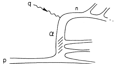
FIG. 4. A resonance-model view of the virtual-photon fragmentation region. The hadron state \{n\} consists of the struck parton plus several wee partons of the target.
